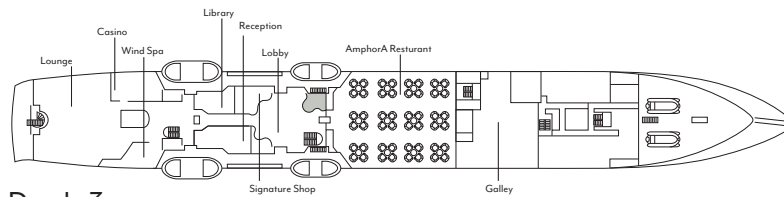
Deck 3
