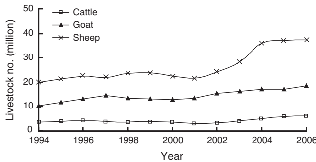
Fig. 2. Livestock numbers from 1994 to 2006 in Inner Mongolia (derived from the Inner Mongolia Rural Economy Statistical Yearbook, from 1994 to 2006).
