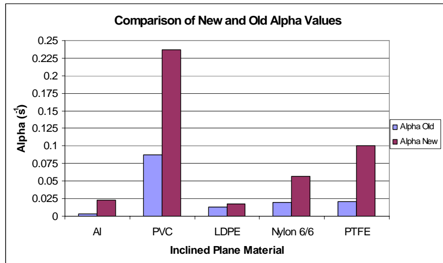
Fig. 2. Comparison of new and old values of the charge generation constant \alpha .
