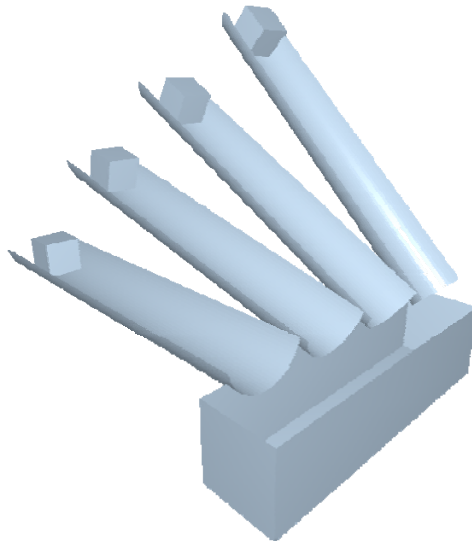
Figure 5. EDEM Model of four inclined curved surfaces at 0°, 15°, 30°, and 45°. Box structures on the end are the particle factories.
