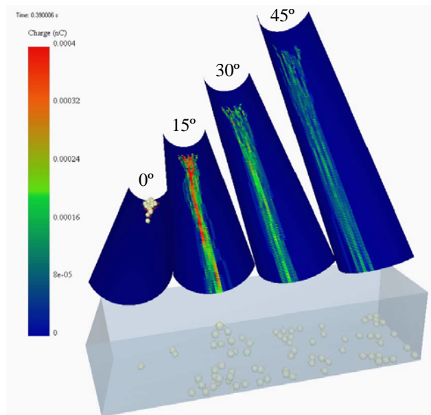
Figure 6. Charge build-up on the inclined surfaces at 0°, 15°, 30°, and 45°.
